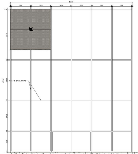
ST 01 FRONT VIEW DETAILS
