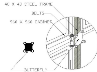
ST 03 BACK SUPPORT DETAILS
