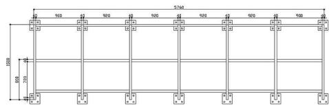
ST 04 TOP VIEW DETAILS
