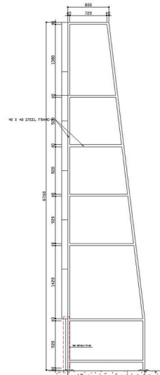
ST 02 SIDE VIEW DETAILS
